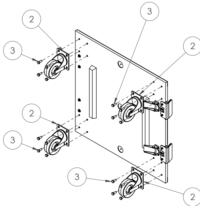
Evo6EH packed with wheel board, but without wheels fitted. Each wheel requires 4 x M8 x 20mm hex bolts (17mm) (supplied). We suggest using a contact adhesive on the bolt thread to secure bolts.
